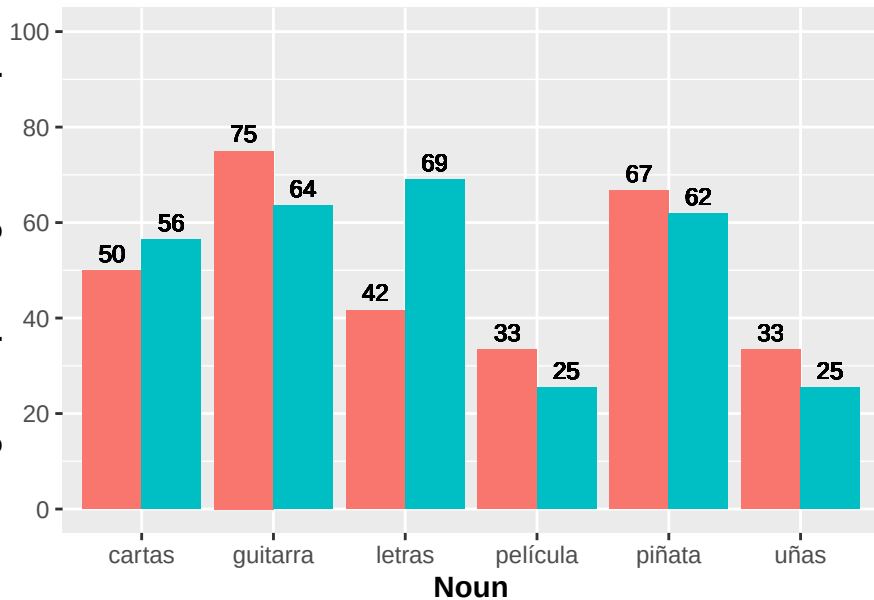
Clitic Gender Selection by Item (Feminine Nouns)
